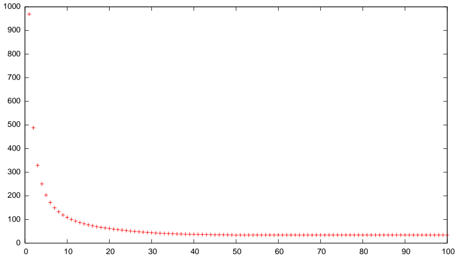
Ropelength vs 100 \times \text{Factor} , 8.21
