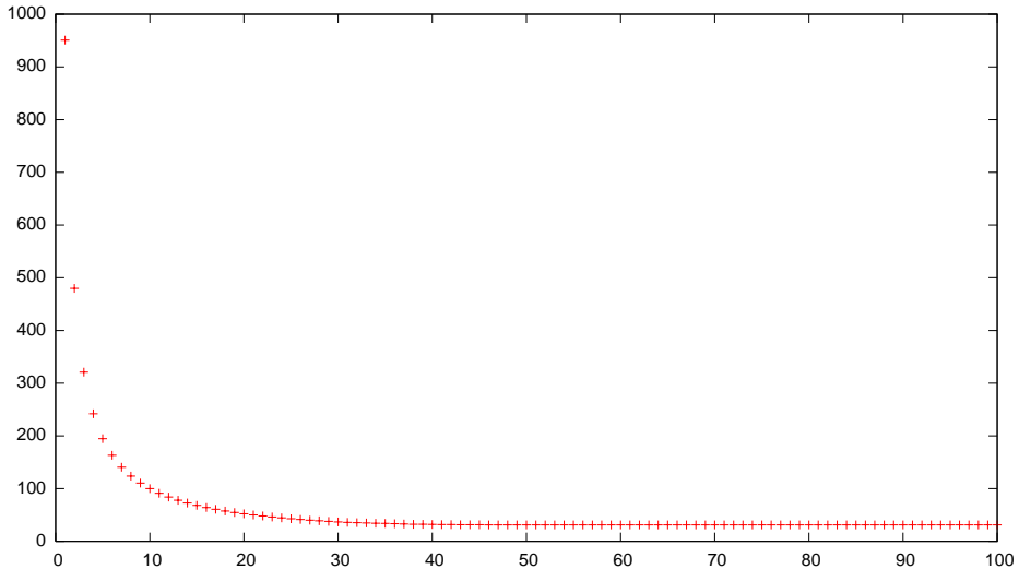
Ropelength vs 100 \cdot \text{Factor} , 8.19
